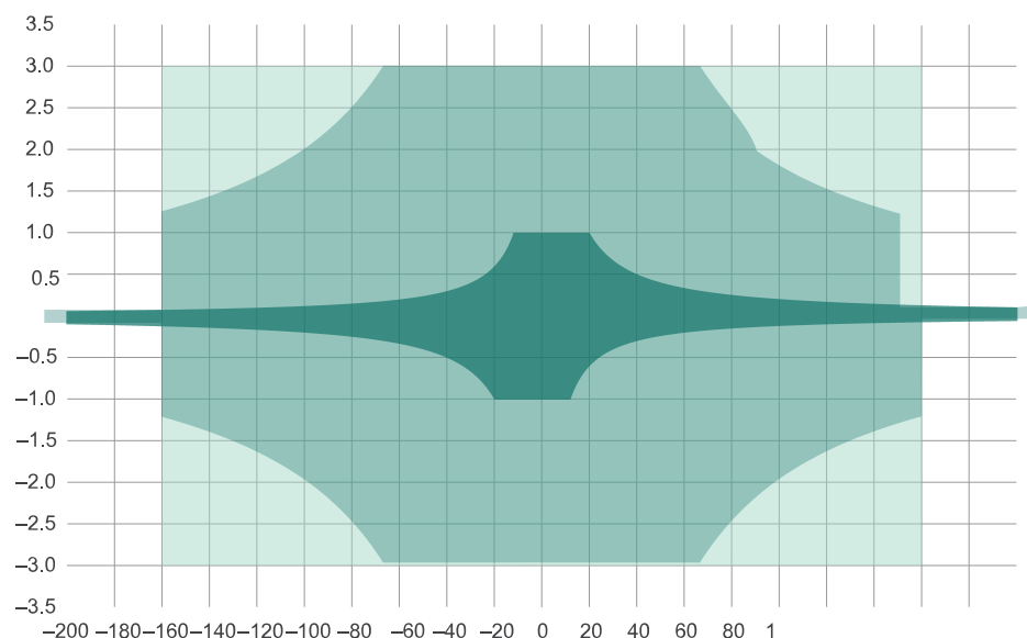
Figure 2. Quadrant Diagram for PXle-4135 (20W)
