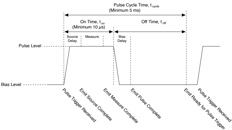
Figure 8. Definition of Pulsing Terminology
