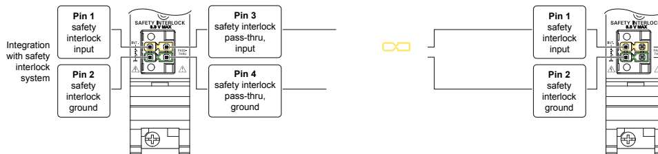
Figure 24. Safety Interlock Pass-Thru Connection
