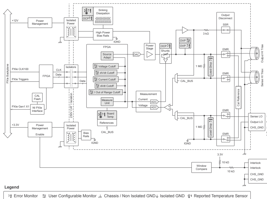
Figure 3. PXIe-4135 Block Diagram
