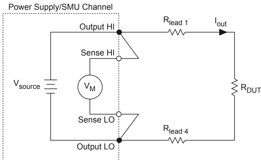
Figure 10. Connecting Local Sense Hardware with a Remote Sense Channel Configuration
