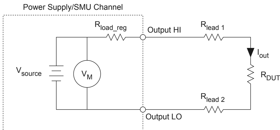
Figure 9. Connecting Signals for Local Sense Measurement
