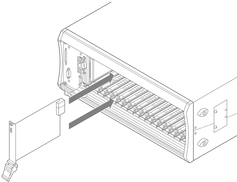
Figure 8. Module Installation
