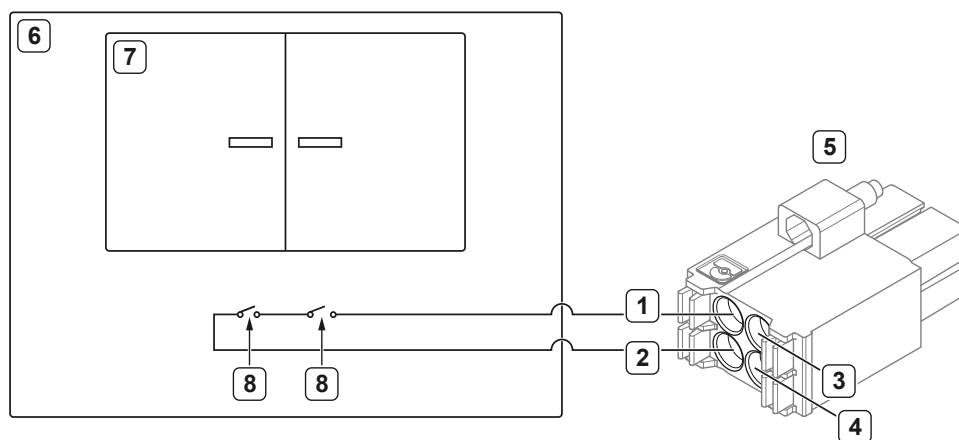
Figure 23. Archetypal Safety Interlock System Design
