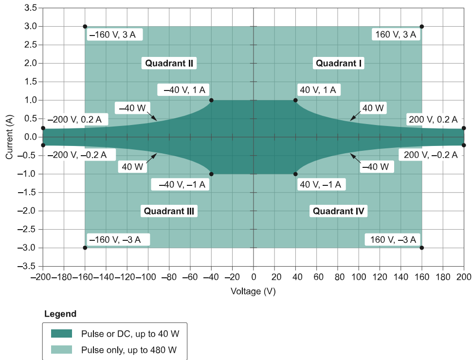
Figure 2. PXIe-4135 (40W) Quadrant Diagram
