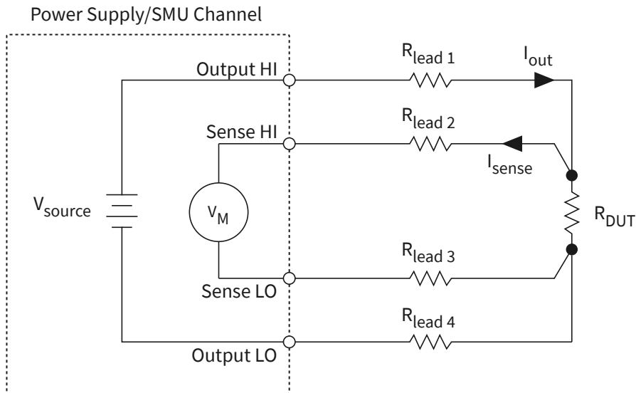
Figure 11. Connecting for a Remote Sense Measurement
