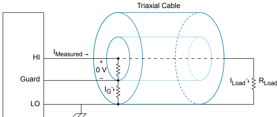
Figure 13. Reducing Leakage with Guarding ( I_{\text{Measured}} = I_{\text{Load}} )
