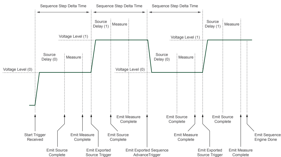
Figure 21. Sequence Step Delta Time Source Model
