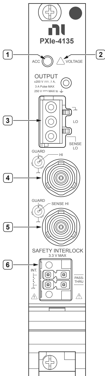
Figure 4. PXIe-4135 Front Panel
