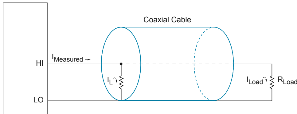
Figure 12. Leakage without Guarding ( I_{\text{Measured}} = I_{\text{Load}} + I_{\text{L}} )
