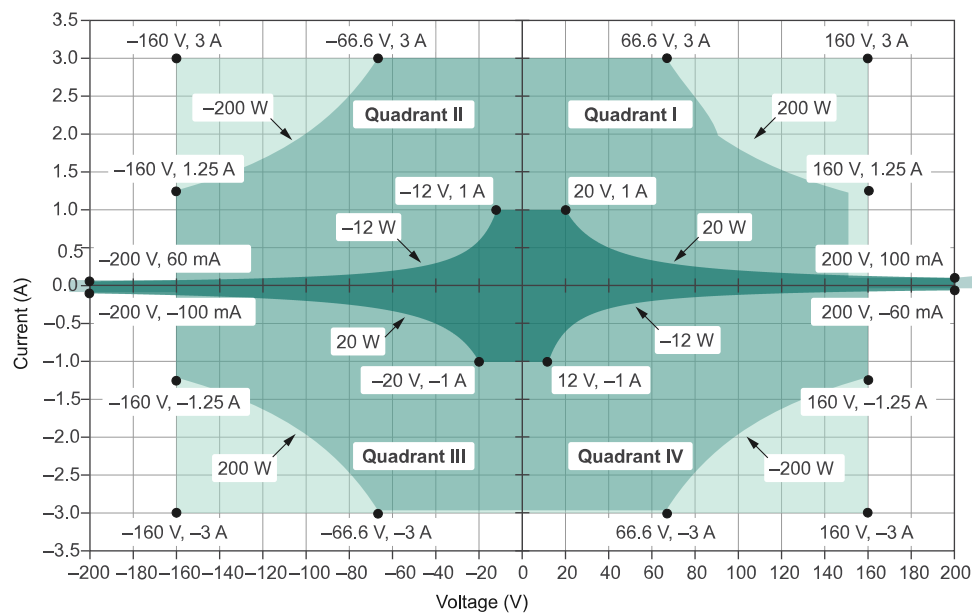
Figure 1. PXIe-4135 (20W) Quadrant Diagram
