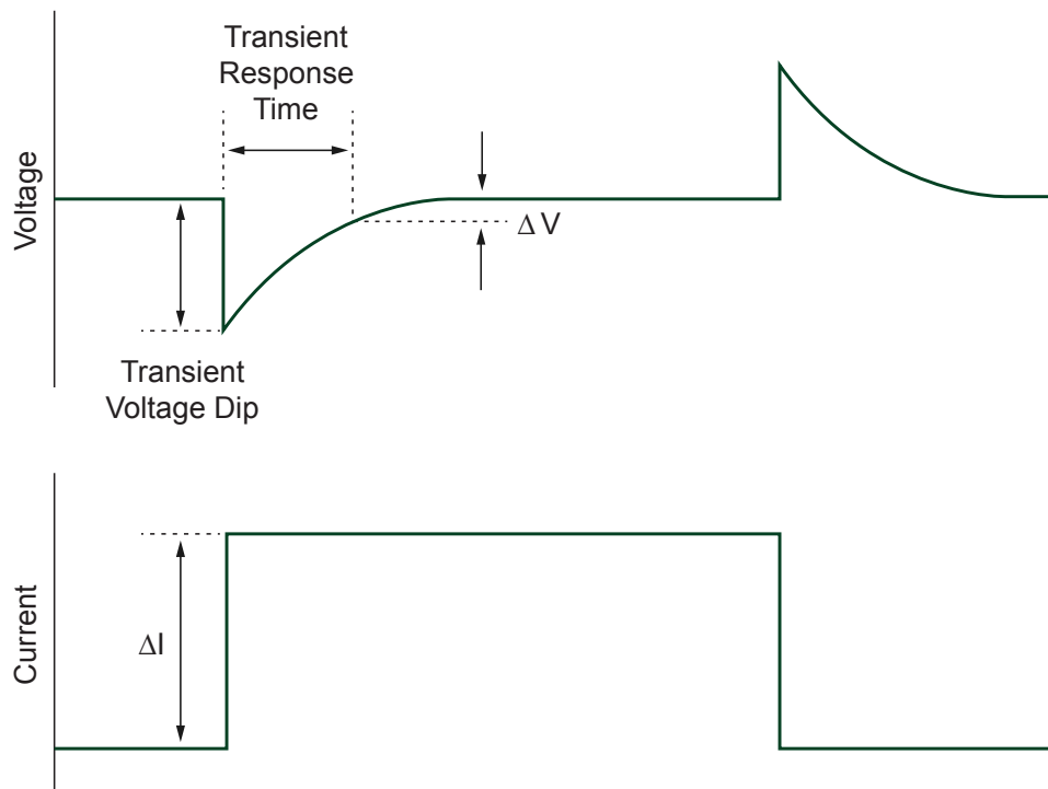
Figure 16. Transient Response
