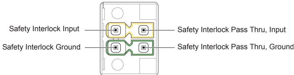
Figure 25. Safety Interlock Input Connector Pinout
