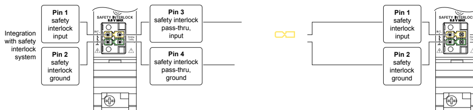
Figure 26. Safety Interlock Pass-Thru Connection
